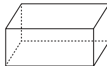
prism
